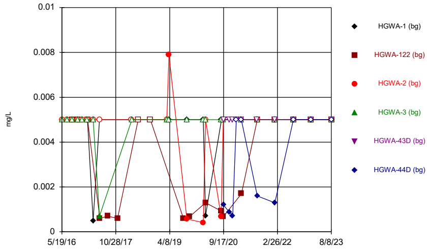
Constituent: Chromium Analysis Run 10/25/2023 6:22 PM View: Time Series & Box Plot Plant Hammond Client: Southern Company Data: Hammond AP-3
