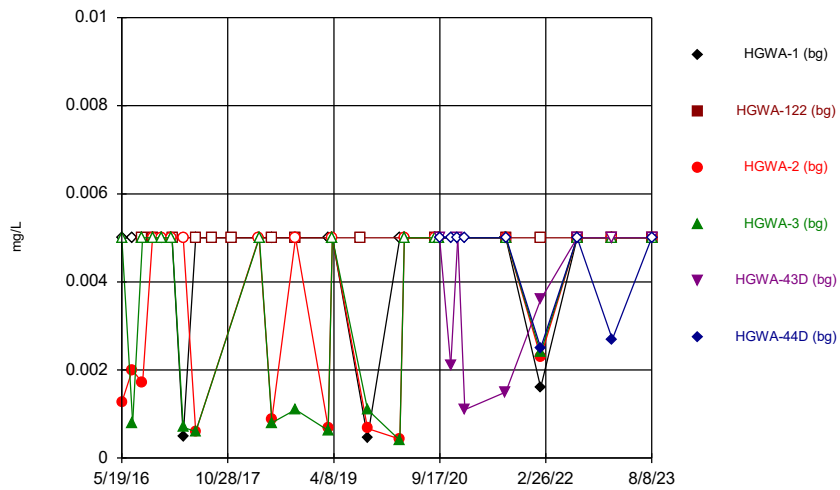
Constituent: Arsenic Analysis Run 10/25/2023 6:22 PM View: Time Series & Box Plot Plant Hammond Client: Southern Company Data: Hammond AP-3
