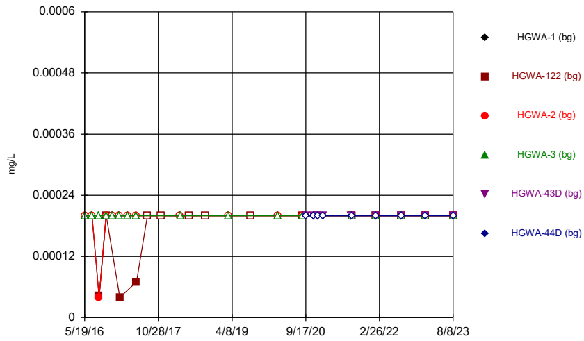
Constituent: Mercury Analysis Run 10/25/2023 6:22 PM View: Time Series & Box Plot Plant Hammond Client: Southern Company Data: Hammond AP-3
