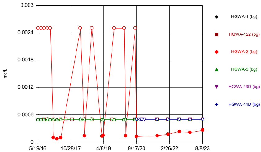
Constituent: Cadmium Analysis Run 10/25/2023 6:22 PM View: Time Series & Box Plot Plant Hammond Client: Southern Company Data: Hammond AP-3
