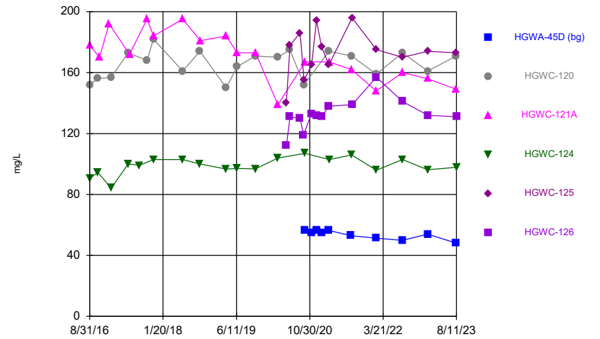
Constituent: Calcium Analysis Run 10/25/2023 6:22 PM View: Time Series & Box Plot Plant Hammond Client: Southern Company Data: Hammond AP-3
