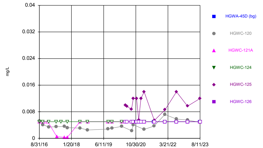
Constituent: Cobalt Analysis Run 10/25/2023 6:22 PM View: Time Series & Box Plot Plant Hammond Client: Southern Company Data: Hammond AP-3
