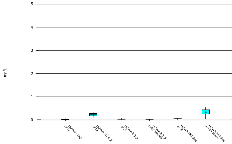
Constituent: Boron Analysis Run 10/25/2023 6:23 PM View: Time Series & Box Plot Plant Hammond Client: Southern Company Data: Hammond AP-3
