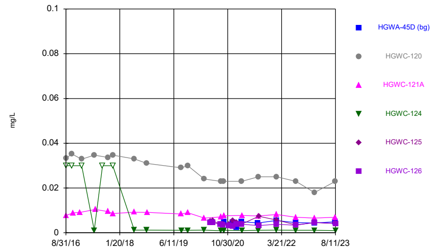
Constituent: Lithium Analysis Run 10/25/2023 6:22 PM View: Time Series & Box Plot Plant Hammond Client: Southern Company Data: Hammond AP-3
