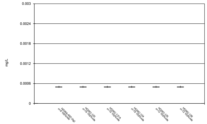
Constituent: Cadmium Analysis Run 10/25/2023 6:24 PM View: Time Series & Box Plot Plant Hammond Client: Southern Company Data: Hammond AP-3
