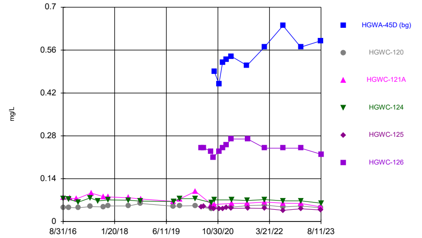
Constituent: Barium Analysis Run 10/25/2023 6:22 PM View: Time Series & Box Plot Plant Hammond Client: Southern Company Data: Hammond AP-3
