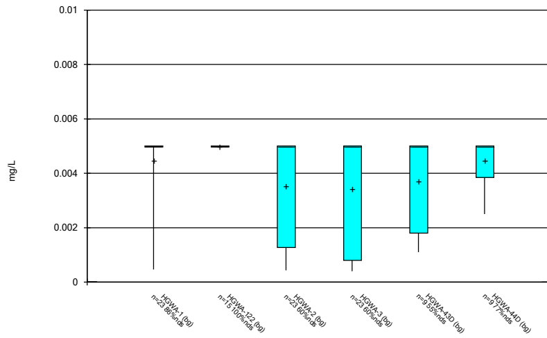
Constituent: Arsenic Analysis Run 10/25/2023 6:23 PM View: Time Series & Box Plot Plant Hammond Client: Southern Company Data: Hammond AP-3
