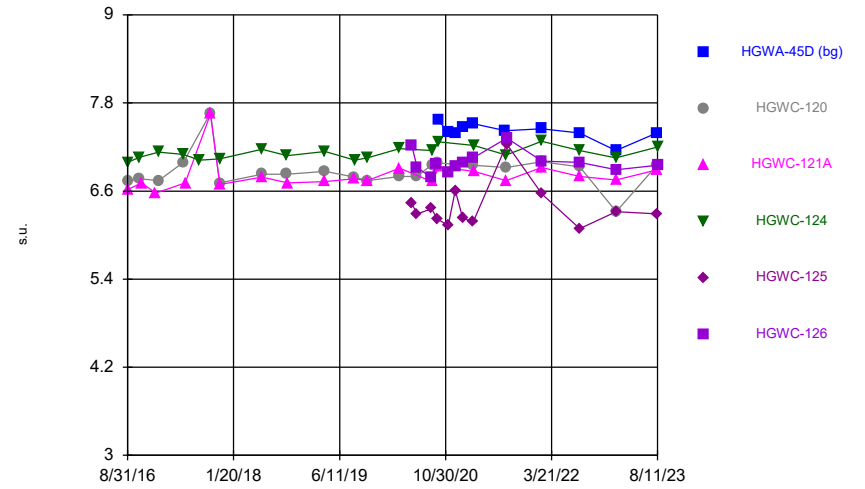
Constituent: pH Analysis Run 10/25/2023 6:22 PM View: Time Series & Box Plot Plant Hammond Client: Southern Company Data: Hammond AP-3
