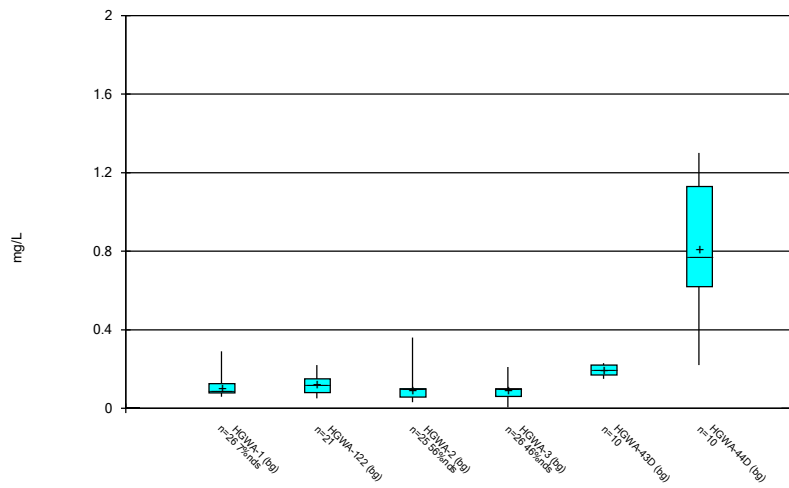
Constituent: Fluoride Analysis Run 10/25/2023 6:24 PM View: Time Series & Box Plot Plant Hammond Client: Southern Company Data: Hammond AP-3
