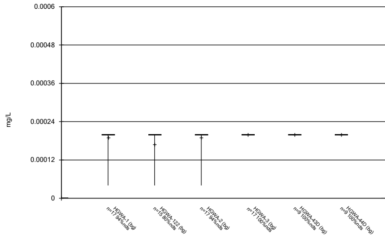
Constituent: Mercury Analysis Run 10/25/2023 6:24 PM View: Time Series & Box Plot Plant Hammond Client: Southern Company Data: Hammond AP-3
