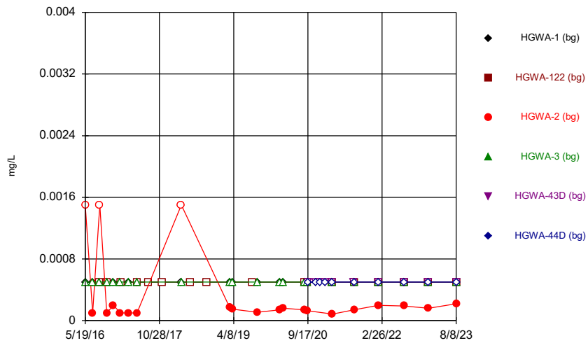
Constituent: Beryllium Analysis Run 10/25/2023 6:22 PM View: Time Series & Box Plot Plant Hammond Client: Southern Company Data: Hammond AP-3
