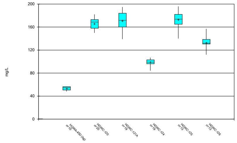
Constituent: Calcium Analysis Run 10/25/2023 6:24 PM View: Time Series & Box Plot Plant Hammond Client: Southern Company Data: Hammond AP-3
