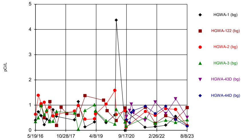
Constituent: Combined Radium 226 + 228 Analysis Run 10/25/2023 6:22 PM View: Time Series & Box Plot Plant Hammond Client: Southern Company Data: Hammond AP-3
