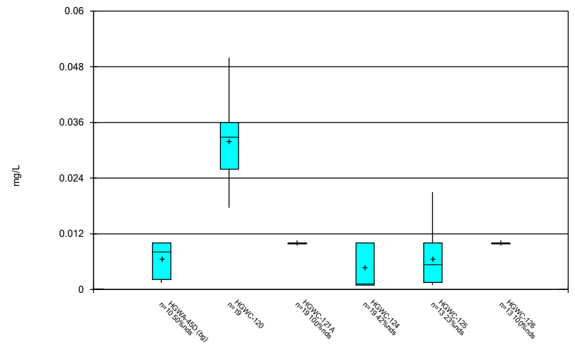
Constituent: Molybdenum Analysis Run 10/25/2023 6:24 PM View: Time Series & Box Plot Plant Hammond Client: Southern Company Data: Hammond AP-3
