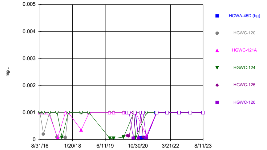
Constituent: Lead Analysis Run 10/25/2023 6:22 PM View: Time Series & Box Plot Plant Hammond Client: Southern Company Data: Hammond AP-3
