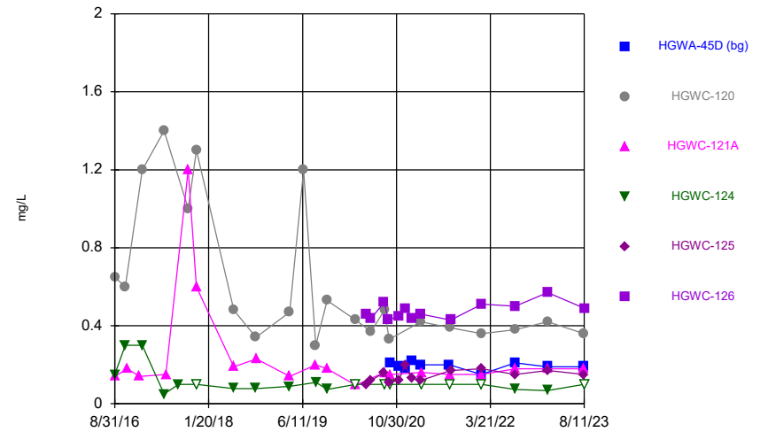
Constituent: Fluoride Analysis Run 10/25/2023 6:22 PM View: Time Series & Box Plot Plant Hammond Client: Southern Company Data: Hammond AP-3
