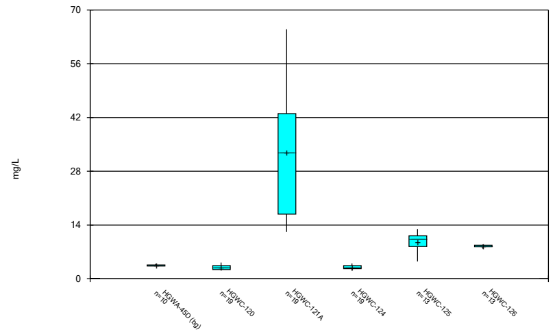
Constituent: Chloride Analysis Run 10/25/2023 6:24 PM View: Time Series & Box Plot Plant Hammond Client: Southern Company Data: Hammond AP-3
