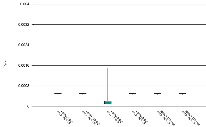
Constituent: Beryllium Analysis Run 10/25/2023 6:23 PM View: Time Series & Box Plot Plant Hammond Client: Southern Company Data: Hammond AP-3
