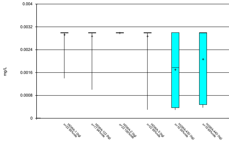
Constituent: Antimony Analysis Run 10/25/2023 6:23 PM View: Time Series & Box Plot Plant Hammond Client: Southern Company Data: Hammond AP-3
