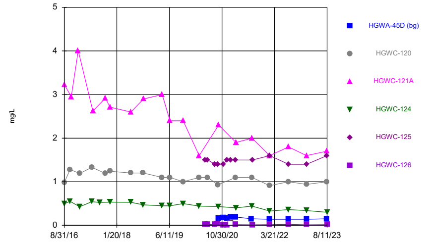
Constituent: Boron Analysis Run 10/25/2023 6:22 PM View: Time Series & Box Plot Plant Hammond Client: Southern Company Data: Hammond AP-3
