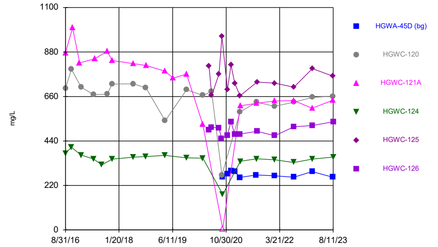
Constituent: Total Dissolved Solids Analysis Run 10/25/2023 6:22 PM View: Time Series & Box Plot Plant Hammond Client: Southern Company Data: Hammond AP-3
