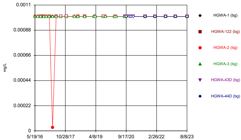
Constituent: Thallium Analysis Run 10/25/2023 6:22 PM View: Time Series & Box Plot Plant Hammond Client: Southern Company Data: Hammond AP-3
