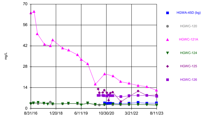
Constituent: Chloride Analysis Run 10/25/2023 6:22 PM View: Time Series & Box Plot Plant Hammond Client: Southern Company Data: Hammond AP-3
