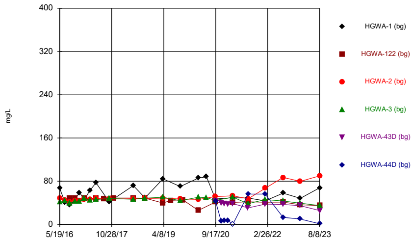
Constituent: Sulfate Analysis Run 10/25/2023 6:22 PM View: Time Series & Box Plot Plant Hammond Client: Southern Company Data: Hammond AP-3
