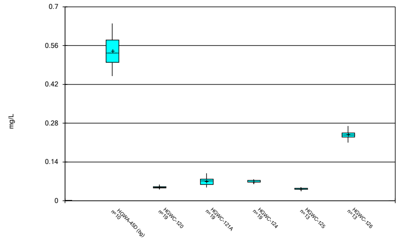
Constituent: Barium Analysis Run 10/25/2023 6:23 PM View: Time Series & Box Plot Plant Hammond Client: Southern Company Data: Hammond AP-3
