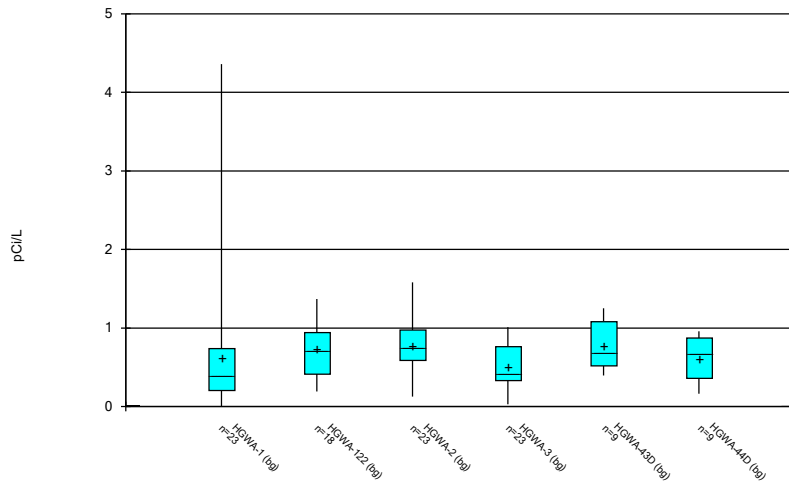
Constituent: Combined Radium 226 + 228 Analysis Run 10/25/2023 6:24 PM View: Time Series & Box Plot Plant Hammond Client: Southern Company Data: Hammond AP-3
