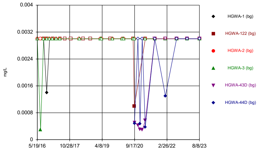
Constituent: Antimony Analysis Run 10/25/2023 6:22 PM View: Time Series & Box Plot Plant Hammond Client: Southern Company Data: Hammond AP-3
