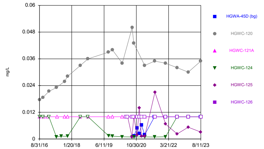
Constituent: Molybdenum Analysis Run 10/25/2023 6:22 PM View: Time Series & Box Plot Plant Hammond Client: Southern Company Data: Hammond AP-3
