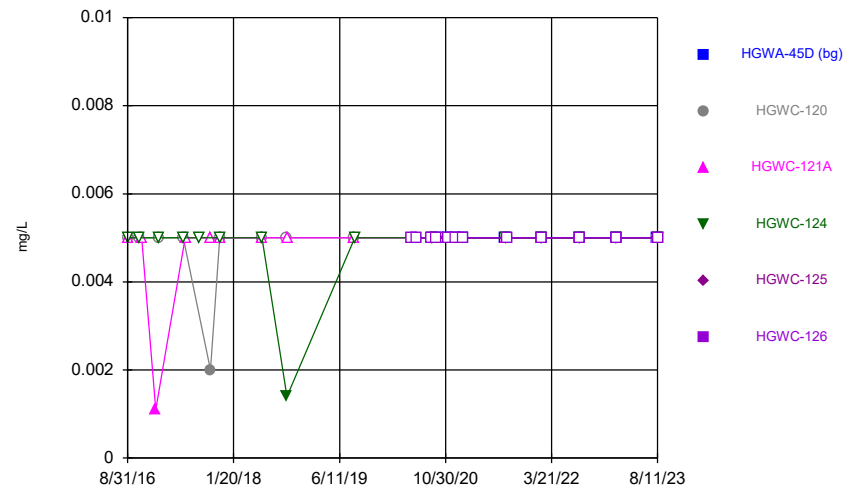
Constituent: Selenium Analysis Run 10/25/2023 6:22 PM View: Time Series & Box Plot Plant Hammond Client: Southern Company Data: Hammond AP-3
