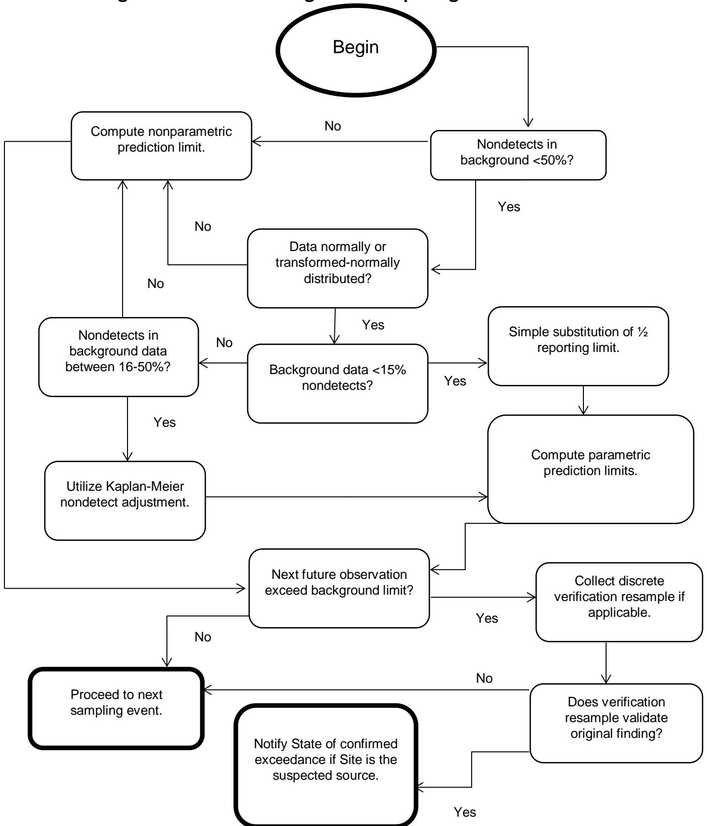
Figure D3 – Decision Logic for Computing Prediction Limits
