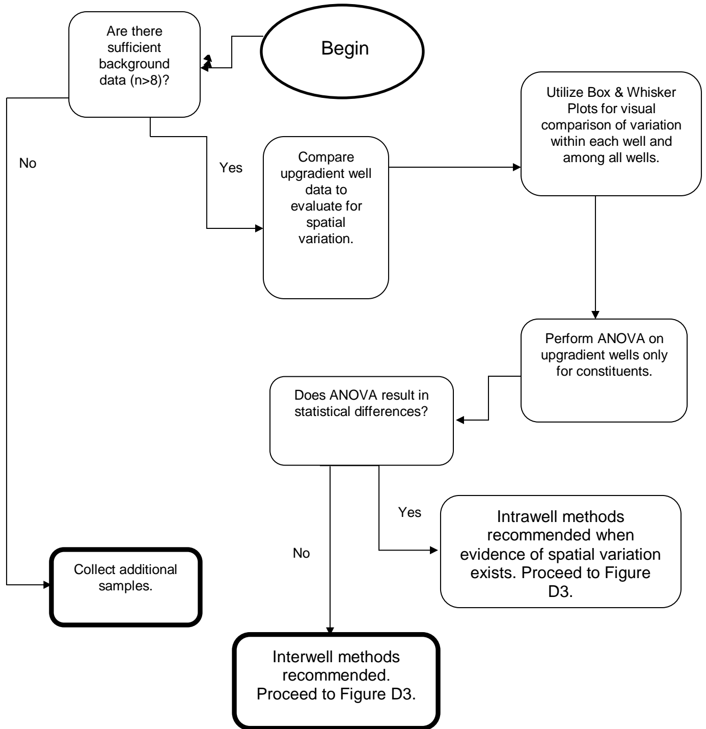
Figure D2 – Decision Logic for Determining Appropriate Statistical Method
